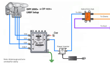
Western Arc International (Single Antenna for Hopper 3)
