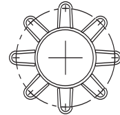
ANCHOR PATTERN 3 2.4 m (8) 3/4" Anchors Equally Spaced on 10.68" Bolt Circle
