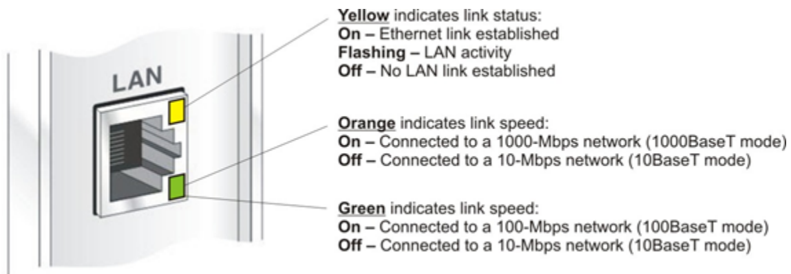
Figure 89: LAN port LEDs
